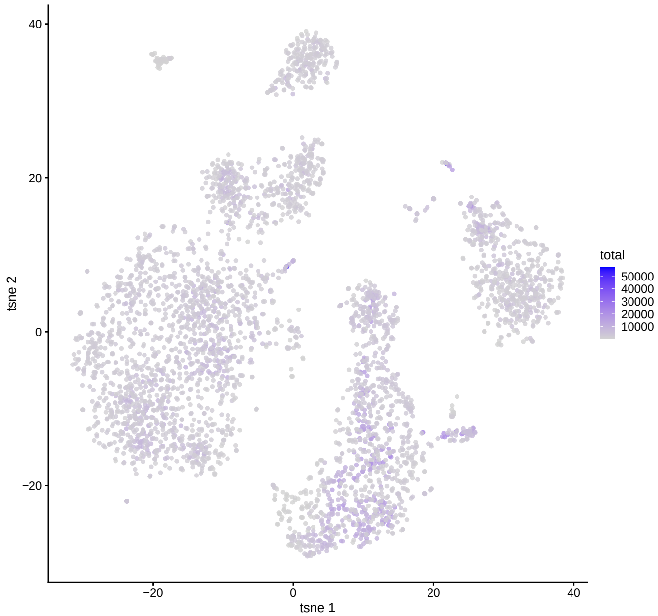
Total number of UMI | TSNE
